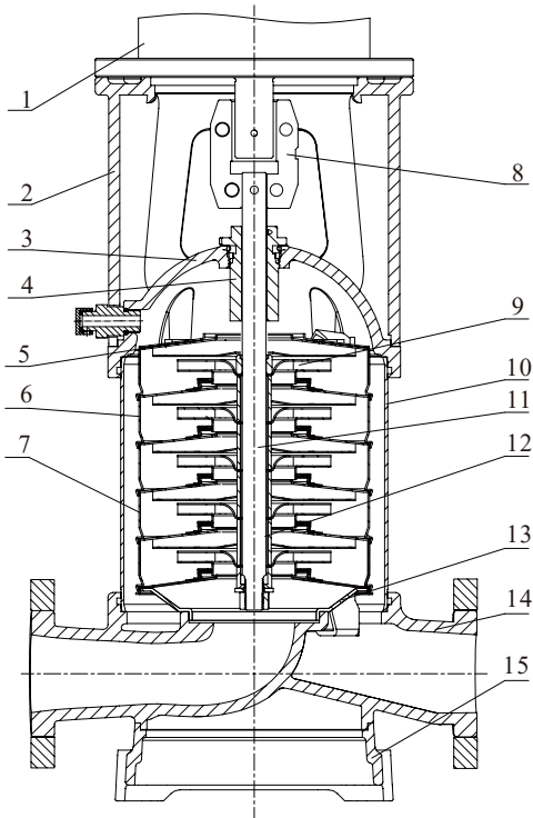
结构图LCS/LCA 8,10,12,15,16,20
