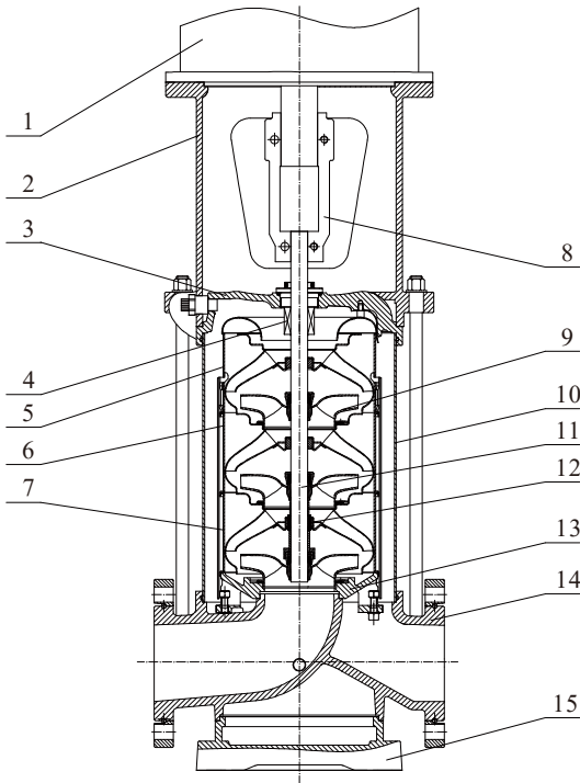
结构图LCS/LCA 100,130,160,190,220,260
